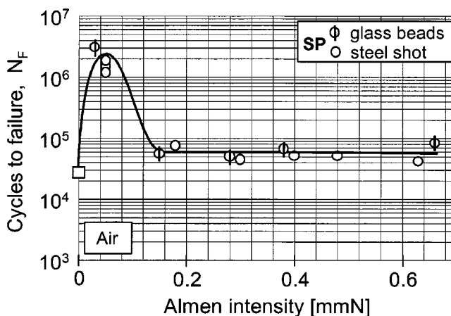
Fig. 8 Fatigue life ( \sigma_a = 175 MPa) vs Almen intensity, effect of peening medium
