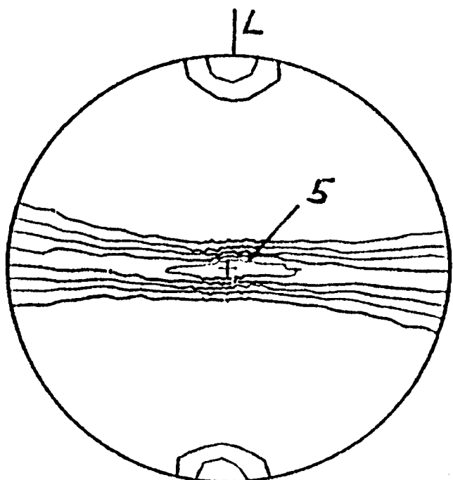
Fig. 2 (0002) pole figure of the as-received bar stock
