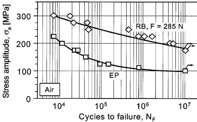
Fig. 14 S-N curves, R = -1 , L direction, air, effect of RB
