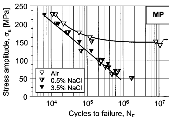
Fig. 7 S-N curves, R = -1 , L direction, effect of environment (MP)
