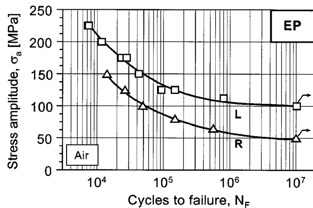
Fig. 4 S-N curves, R = 1 , air, effect of loading direction (EP)
