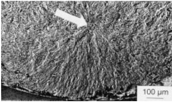
Fig. 13 Subsurface fatigue crack nucleation (SEM), F = 285 N ( RB )
